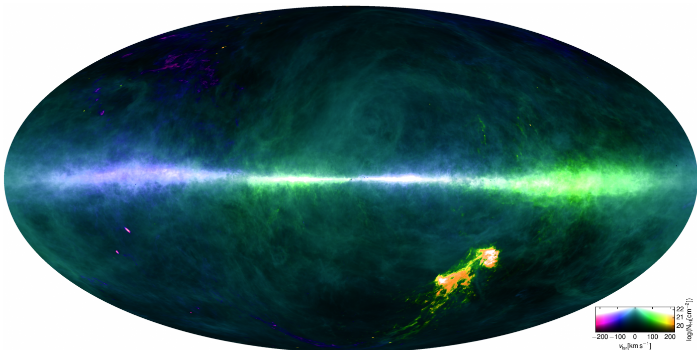
Fig. 3. All-sky composite map of the first two moments of the H I distribution using the same coordinate system and map projection as Fig. 2. The Moment-0 (the column density) determines brightness (log-scale), while the Moment-1 (intensity-weighted radial velocities) is encoded as different hues. The brightness is furthermore modified according to the velocity scale, to render the weaker intermediate- and high-velocity gas more visible. We note that radial velocities in excess of the displayed color scale are subject to clipping: the true radial velocities of red and orange features may be larger than what the colors denote.
