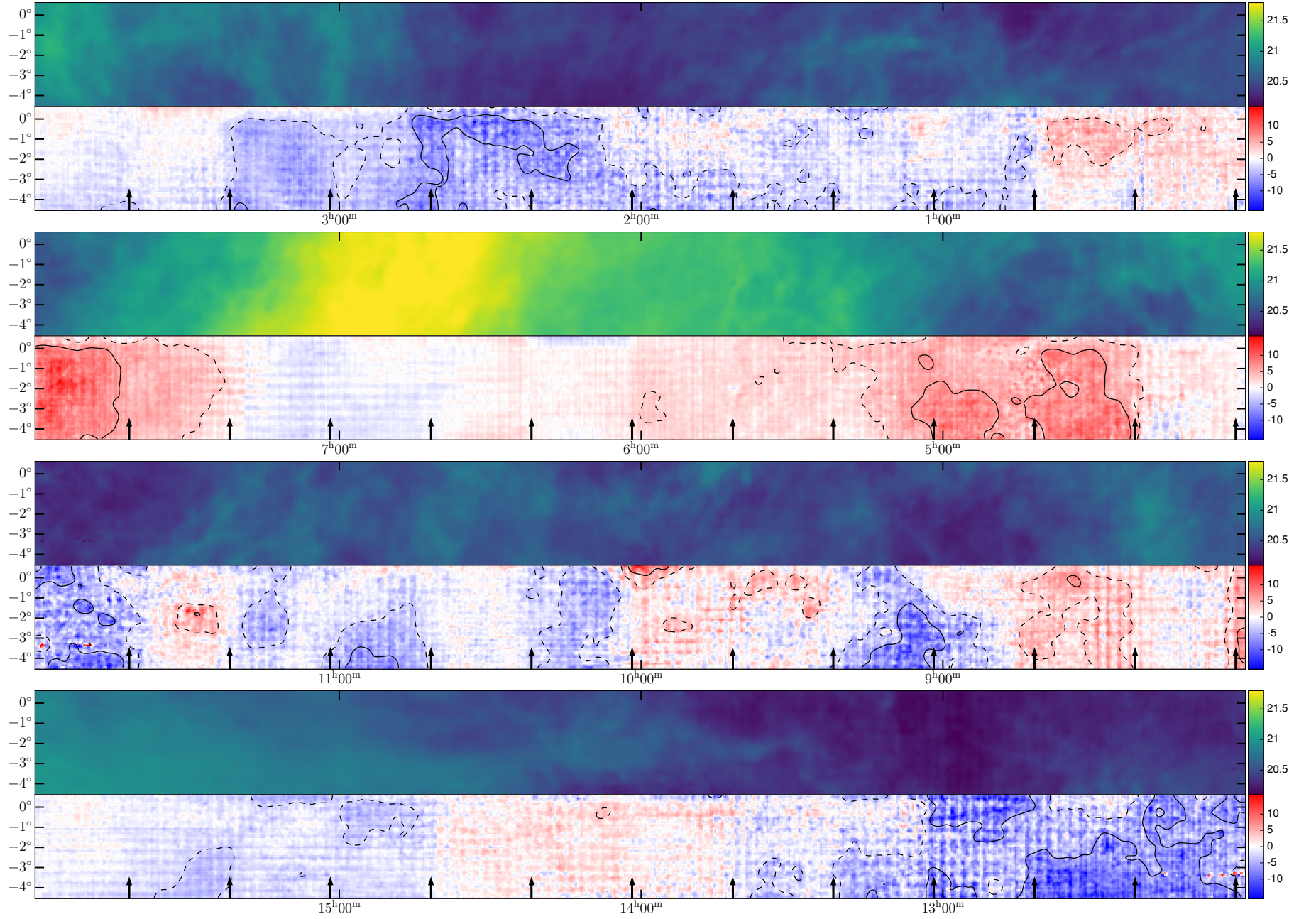
Fig. A.1. EBHIS vs. GASS column densities in the right ascension range 0^{\text{h}} to 16^{\text{h}} . The upper panel in each stripe shows \log(N_{\text{H I}}^{\text{GASS}} [\text{cm}^{-2}]) , the lower panels show the relative difference (N_{\text{H I}}^{\text{EBHIS}} - N_{\text{H I}}^{\text{GASS}}) / N_{\text{H I}}^{\text{EBHIS}} in percent. For convenience, each of the lower panels also contains contour levels for \pm 3\% (dashed lines) and \pm 6\% (solid lines), as well as black arrows to mark the EBHIS field limits.
