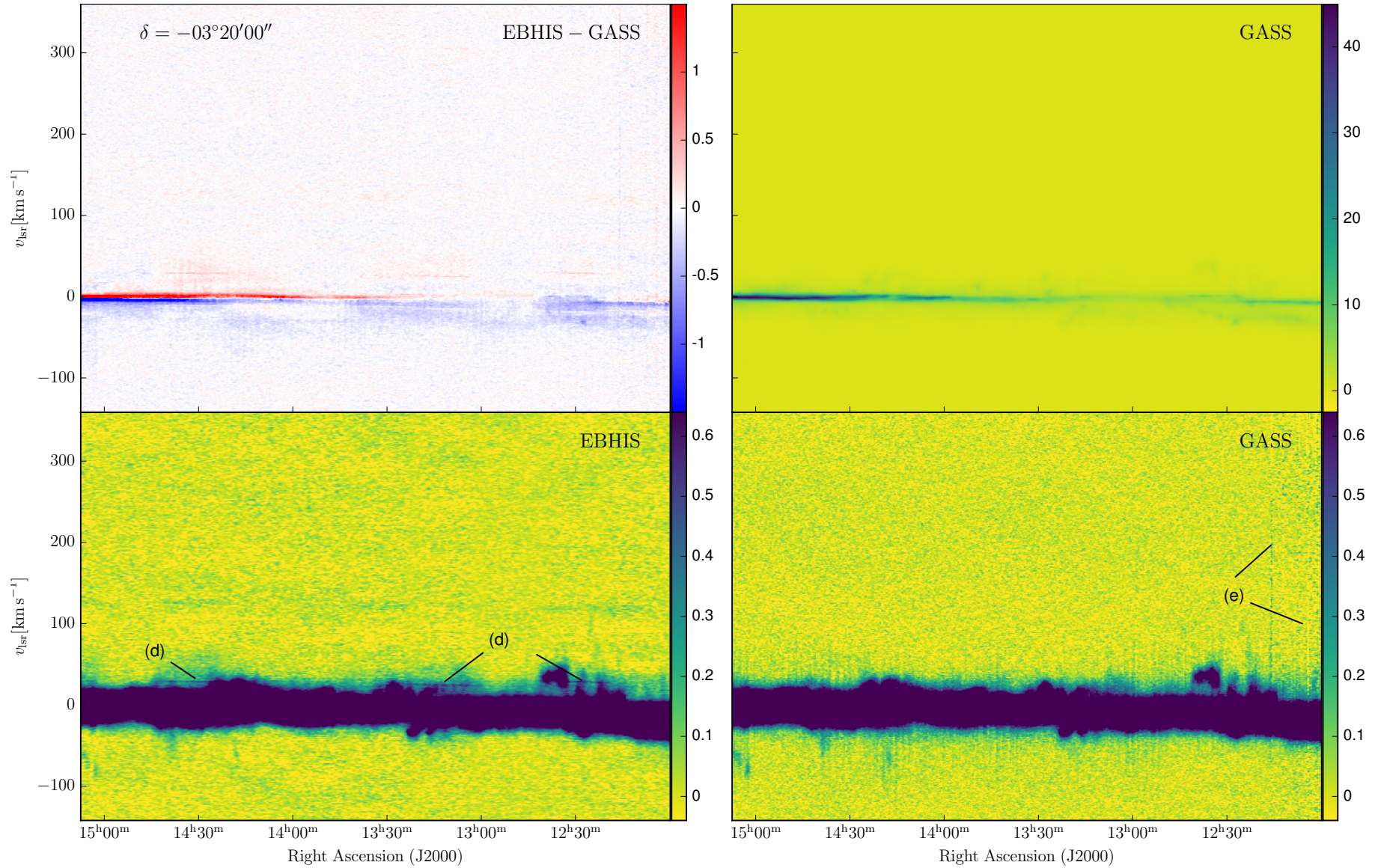
Fig. A.3. As Fig. A.2, showing typical EBHIS and GASS residual RFI features. The labeled features are: (d) narrowband RFI within or very close to the Milky Way disk emission in EBHIS data; (e) rare broadband events, not detected by the GASS RFI flagger. See text for further discussion.
