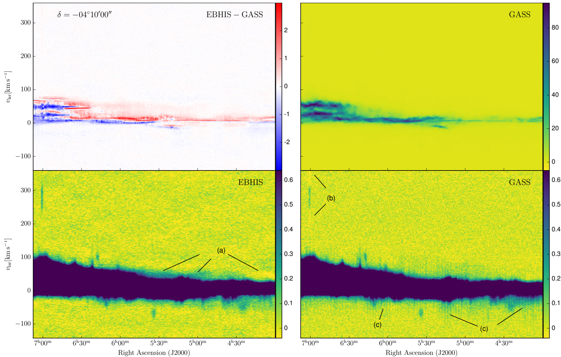
Fig. A.2. Typical EBHIS and GASS baseline problems. The four panels show a position–velocity slice of the overlap-region datacube. Top left panel: difference between EBHIS and GASS, top right panel: GASS data, and bottom panels: EBHIS and GASS data with a zoomed-in intensity scale. The labeled features are: (a) larger-angular scale baseline fluctuations in direct vicinity of the Milky Way disk H I profile in EBHIS data; (b) baseline deficiencies around non-disk objects in GASS, caused by improper flagging; and (c) increase in baseline level associated to the rectangular pattern visible in Fig A.1. All colorbars show brightness temperature, T_B , in units of Kelvin. See text for further discussion.
